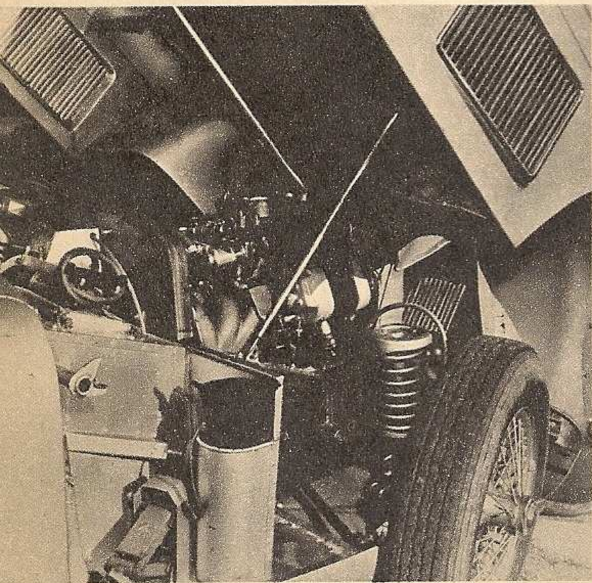
Six-cylinder engine has dual carburetors, double overhead camshaft, is superbly engineered. Hood over the engine, bottom, swings forward in one unit. Note handy tool carrier, center foreground.
